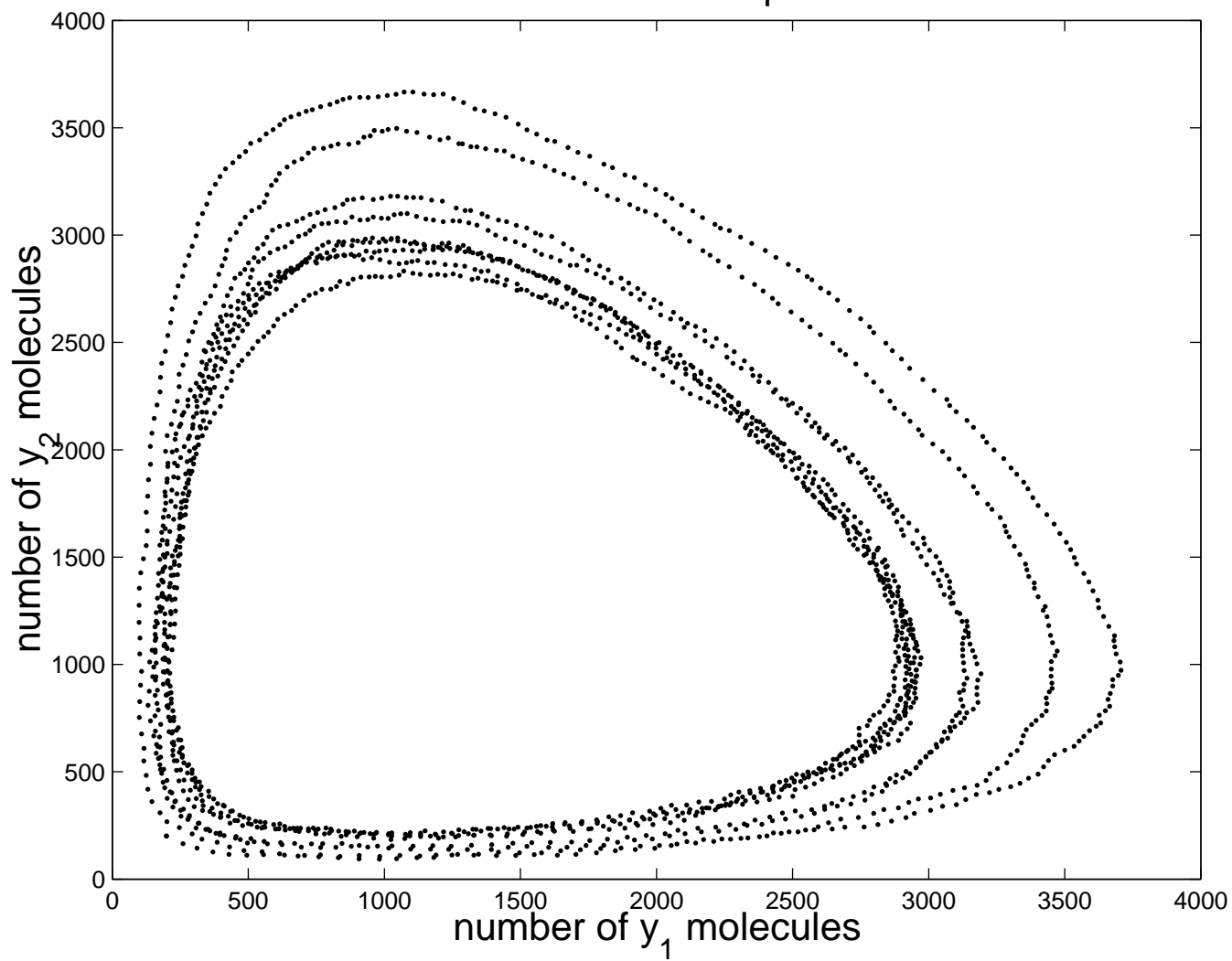
Lotka via Gillespie
