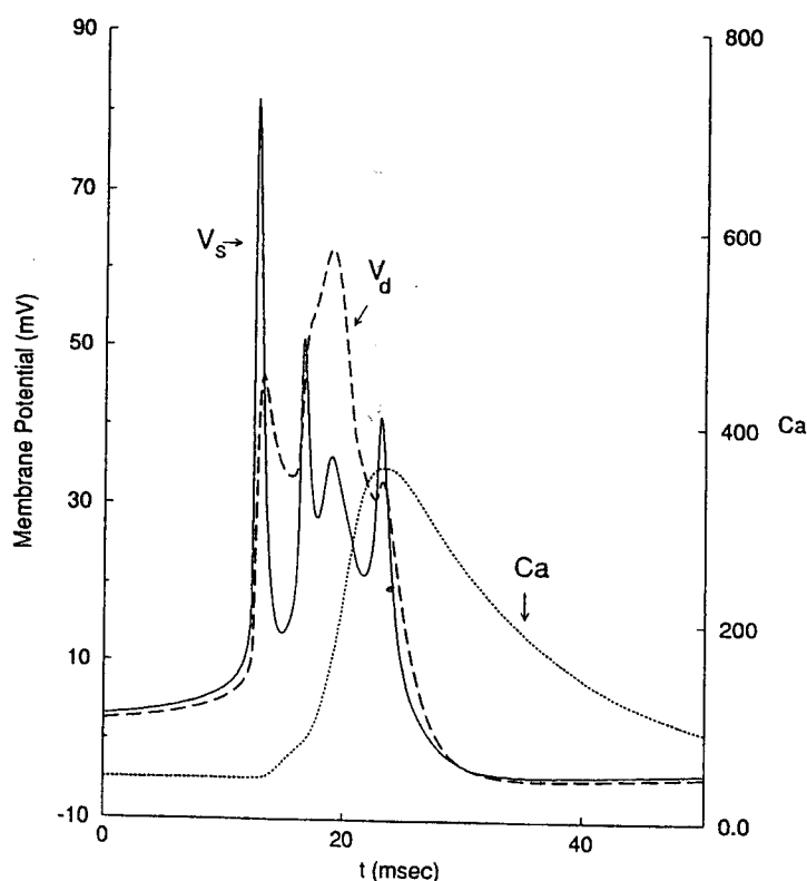
Fig. 3. Time courses of somatic voltage, V_s , dendritic voltage, V_d , and Ca during a burst. Parameters were as in Fig. 2A (note scale for Ca is different than in Fig. 2A). Burst is initiated by somatic action potential which triggers subthreshold dendritic Ca spike. This is followed by full Ca spike in the dendrite leading to somatic burst pattern. Dendritic spike, and hence burst, is terminated by I_{K-C} current which turns on when Ca reaches appreciable levels.
