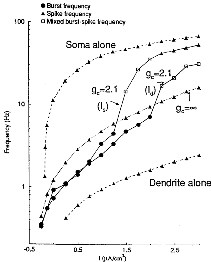
Fig. 5. Frequency current ( f - I ) relation under various coupling regimes. Frequency is determined by the number of times V_s increases past 70 mV (except in the case of the isolated dendrite where we replace V_s with V_d ). Dashed curves show f - I for the isolated soma and for the isolated dendrite; here the I on the abscissa indicates I_s and I_d respectively. Solid curves show f - I for standard coupling parameter values ( g_c = 2.1 mS/cm 2 , p = 0.5 ) in response to I_s (as in Fig. 4) or I_d . Dotted curve shows f - I for g_c = \infty , p = 0.5 ; here the effect of I_s is equivalent to that of I_d . Circles represent burst frequency while triangles represent spike frequencies (somatic spike frequency for soma alone and for g_c = 2.1 , dendritic spike frequency for dendrite alone, and soma-dendritic spike frequency for g_c = \infty ). Squares correspond to solutions with mixtures of bursts and isolated (somatic) spikes; frequency here is combined rate of these events.
