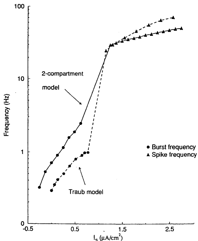
Fig. 6. Frequency versus steady somatic current injection for 2-compartment model ( g_c = 1.85 \text{ mS}/\text{cm}^2 , p = 0.5 ) and for Traub model. Burst frequency is indicated with circles and somatic spike frequency with triangles. Both curves show transition from bursting to spiking as I_s is increased. For Traub model, burst and spike frequency data were taken from Traub et al. (1991, Fig. 10); current in \mu\text{A}/\text{cm}^2 was determined by dividing absolute current by half the area of the Traub neuron.
