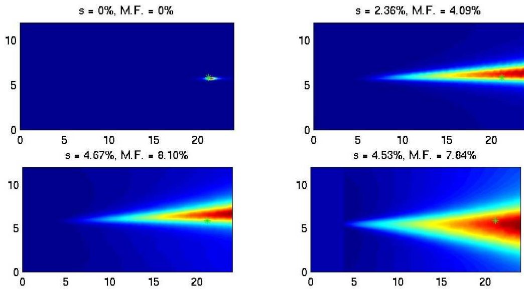
FIG. 7: The DOA estimate [ DOA estimate (15)] of the location of one target in random media with different strength of the fluctuations of the sound speed. The exact location of the target is denoted by the green star. The standard deviation s and maximum fluctuations (M.F.) are indicated on the top of each view. The horizontal axis is the range in mm and the vertical axis is the cross-range in mm.
