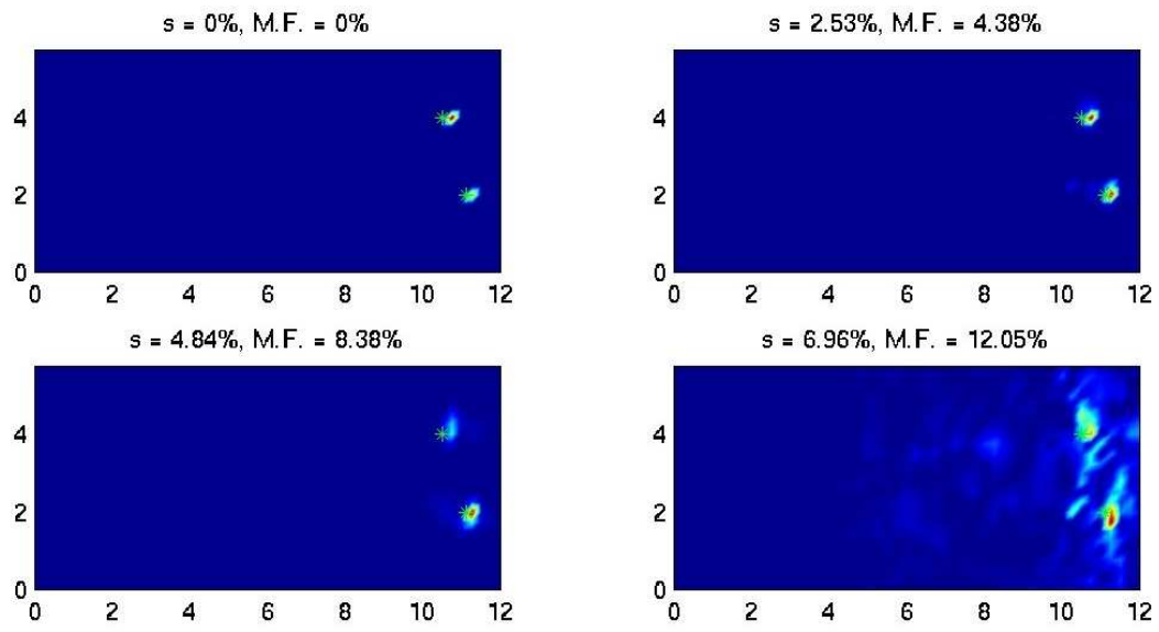
FIG. 14: Same as Fig. 13 with two targets.
