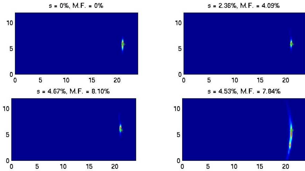
FIG. 11: Combined MF_T and ATSV [ MF_T - ATSV estimate (24)] estimation of one target location in random media with different strength of the fluctuations of the sound speed. The exact location of the target is denoted by the green star. The standard deviation s and maximum fluctuations (M.F.) are indicated on the top of each view. The horizontal axis is the range in mm and the vertical axis is the cross-range in mm.
