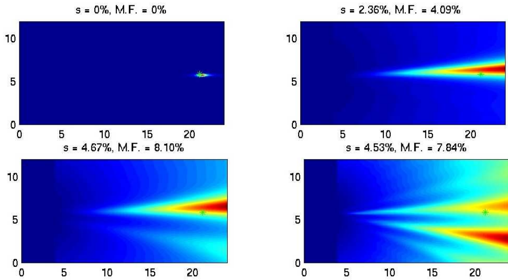
FIG. 3: The MUSIC central frequency estimate [ MUSIC estimate (10)] of the location of one target in random media with different strength of the fluctuations of the sound speed. The exact location of the target is denoted by the green star. The standard deviation s and maximum fluctuations (M.F.) are indicated on the top of each view. The horizontal axis is the range in mm and the vertical axis is the cross-range in mm.
