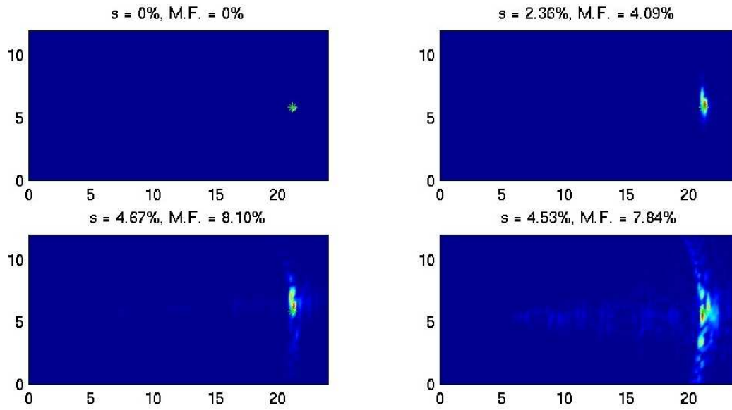
FIG. 13: Combined DOA and SAI [ DOA - SAI estimate (26)] estimation of one target location in random media with different strength of the fluctuations of the sound speed. The exact location of the target is denoted by the green star. The standard deviation s and maximum fluctuations (M.F.) are indicated on the top of each view. The horizontal axis is the range in mm and the vertical axis is the cross-range in mm.
