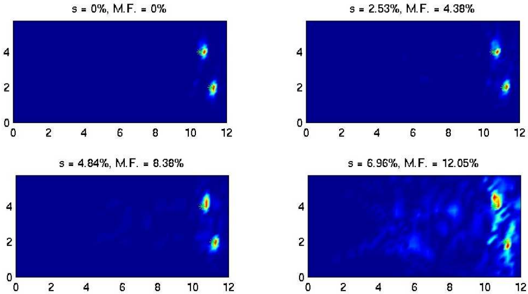
FIG. 10: Similar to Fig. 9 but with two targets .
