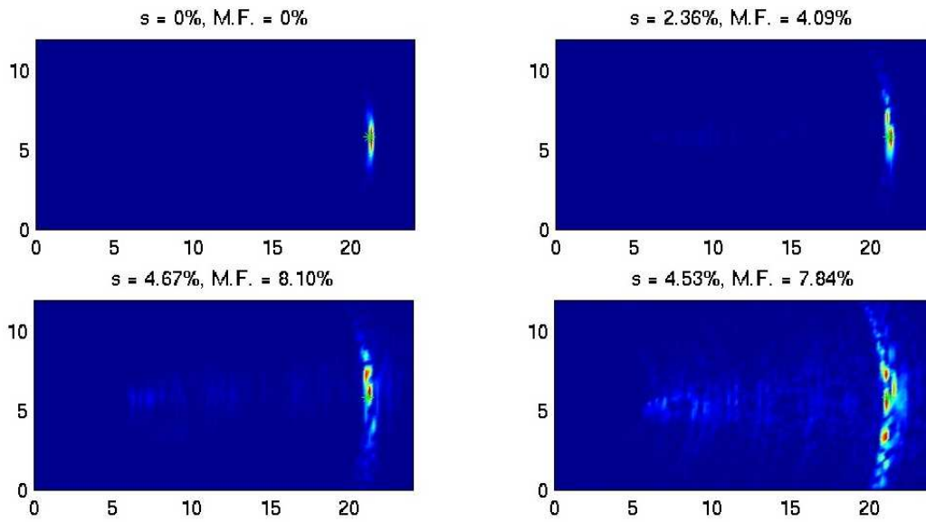
FIG. 9: Combined MF_T and SAI [ MF_T - SAI estimate (18)] estimation of the location of one target in random media with different strength of the fluctuations of the sound speed. The exact location of the target is denoted by the green star. The standard deviation s and maximum fluctuations (M.F.) are indicated on the top of each view. The horizontal axis is the range in mm and the vertical axis is the cross-range in mm.
