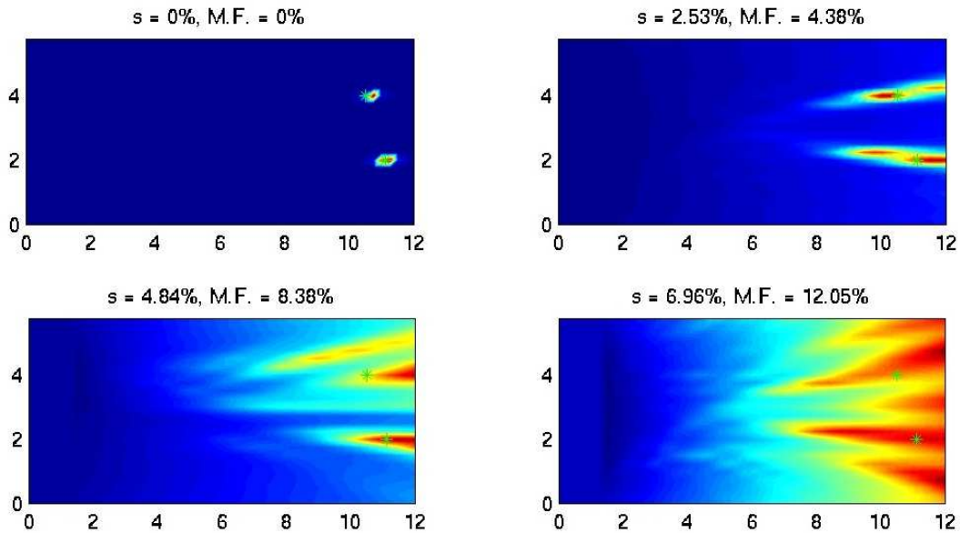
FIG. 4: Similar to Fig. 3 but with two targets.
