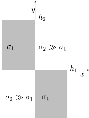
Figure 3.6: Rectangular checkerboard
