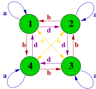
FIG. 1 Graph of a four gene network with circulant A
