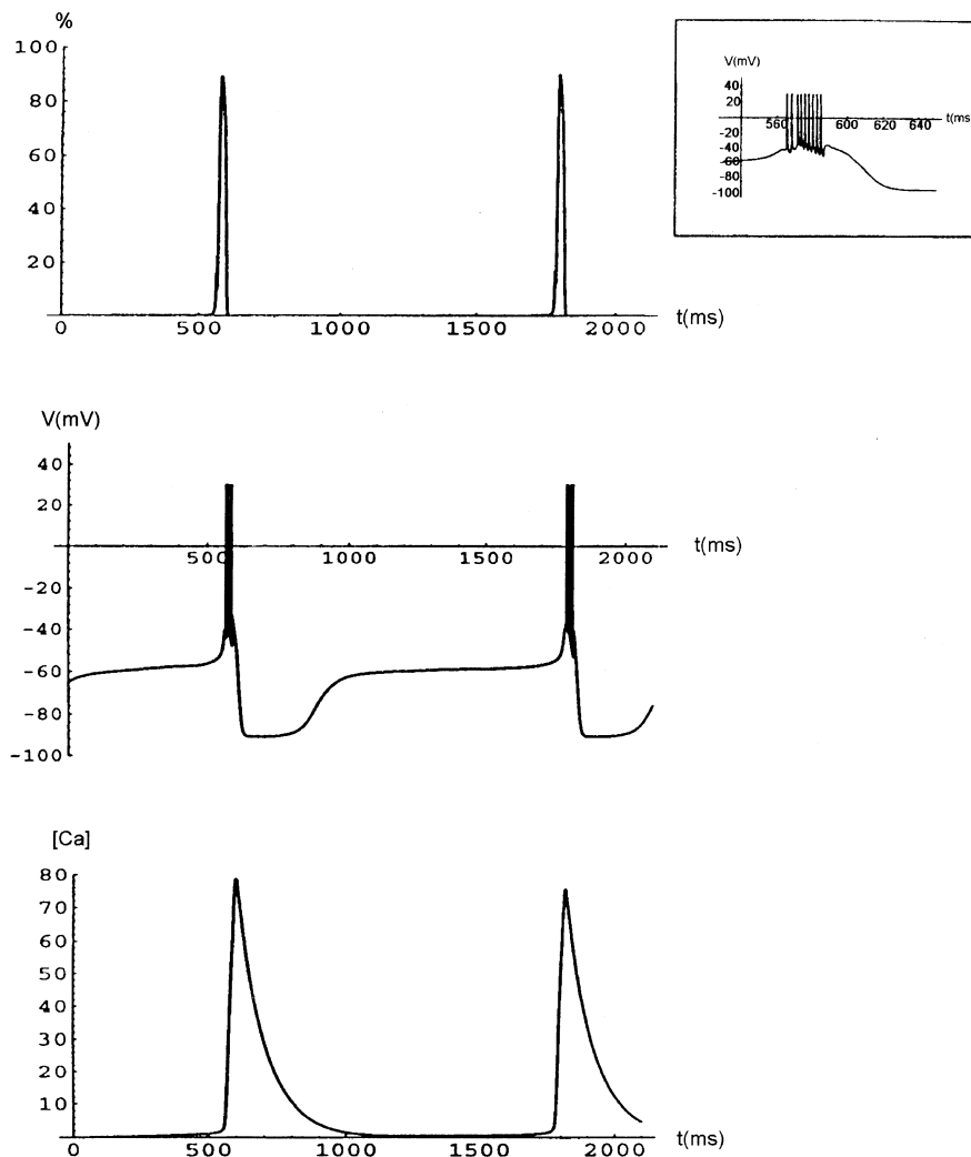
Fig. 1. Fully synchronized population burst ( \gamma_{\text{FP}} = 0.01825 \text{ mS cm}^{-2} , I_{\text{ext}} = 0.09 \mu\text{A cm}^{-2} ): the behavior of pyramidal cells (cf. Traub et al. 1992; Fig. 4/B1). Top: percentage of firing cells in the population. Middle: membrane potential of an 'average cell'; the burst form is shown in the inset . Bottom: calcium concentration of the 'average cell'
