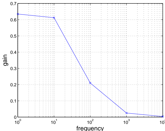
Figure 2.10 The membrane circuit behaves like a low-pass filter. Compare to Figure 2.8.
