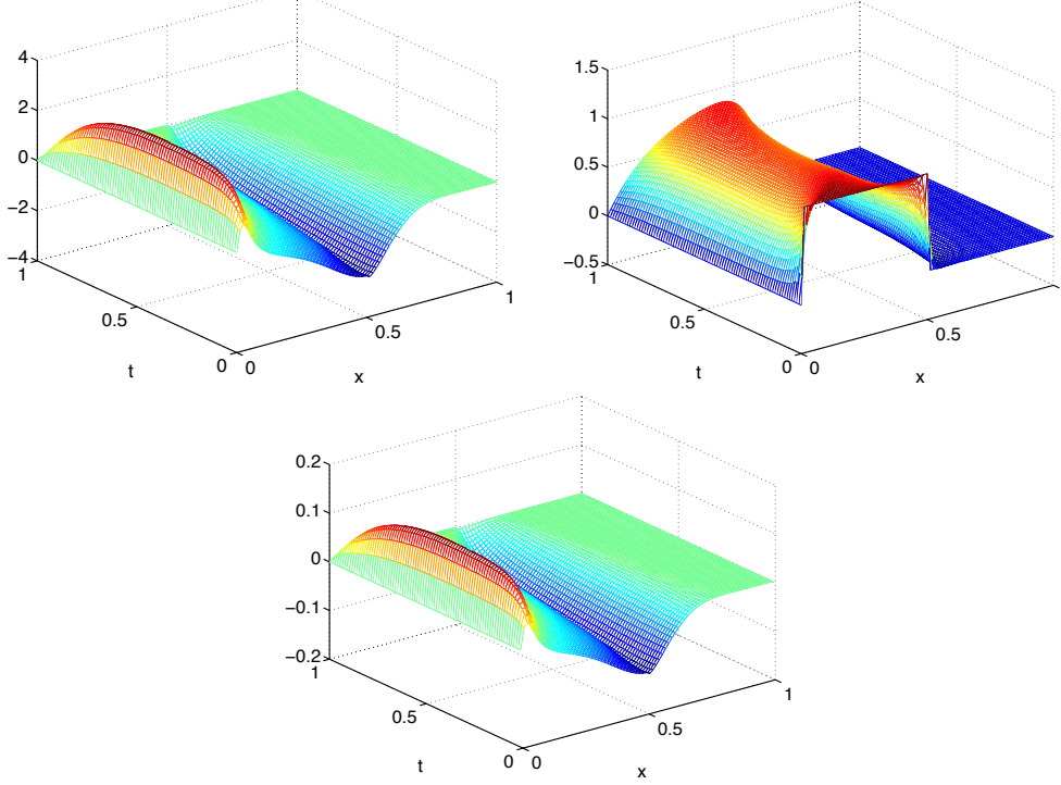
FIG. 5.3. Optimal control u_* (upper left), corresponding solution y(u_*) of Burgers' equation (upper right) and corresponding Lagrange multipliers \lambda(u_*) (bottom)
