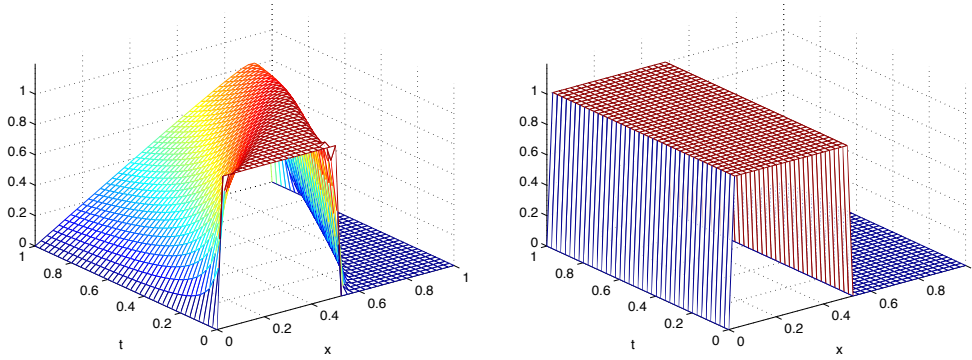
FIG. 5.2. Solution of Burgers' equation with u = 0 (no control) (left) and desired state z (right)
