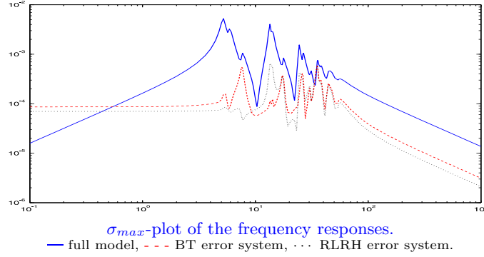
Building model N = 48 , m = p = 1 , n = 10
