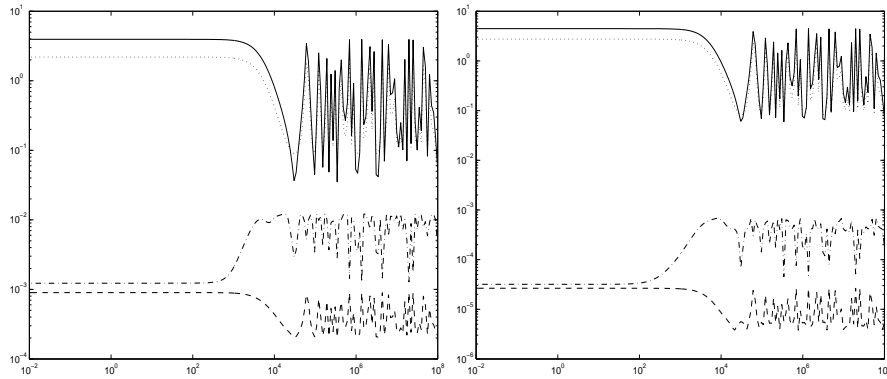
Fig.2a,b: — full model, \cdots approx. errors (20 steps), -\cdot- approx. errors (60 steps), -- approx.errors (exact gramian)
