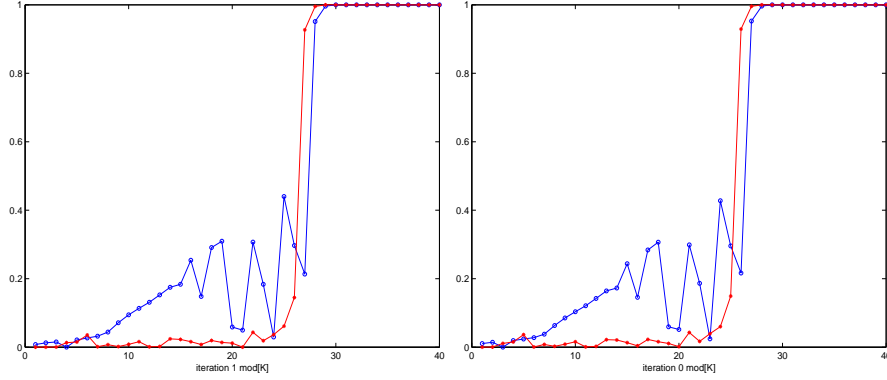
Fig.1a,b: \circ — \cos(\angle(S_k, S_{k-2})) , \ast — \cos(\angle(S_k, S_\infty)) for odd and even k
