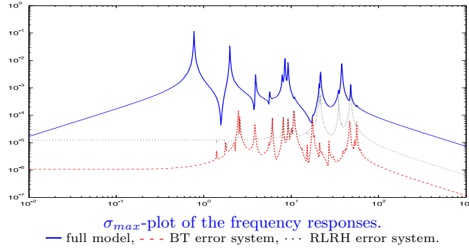
ISS model N = 270 , m = p = 3 , n = 32
