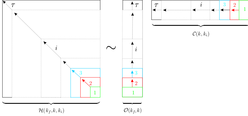
Fig.3: Submatrix sequence approximated by low rank approximations
