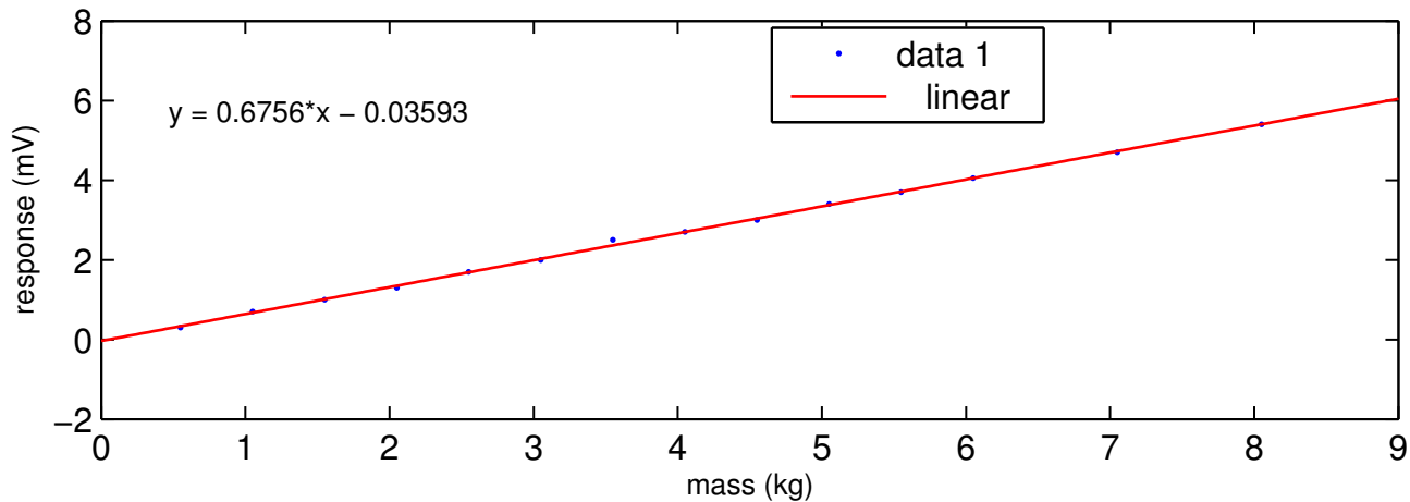
Force transducer calibration
